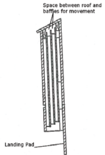
Interior of a maternity bat house
