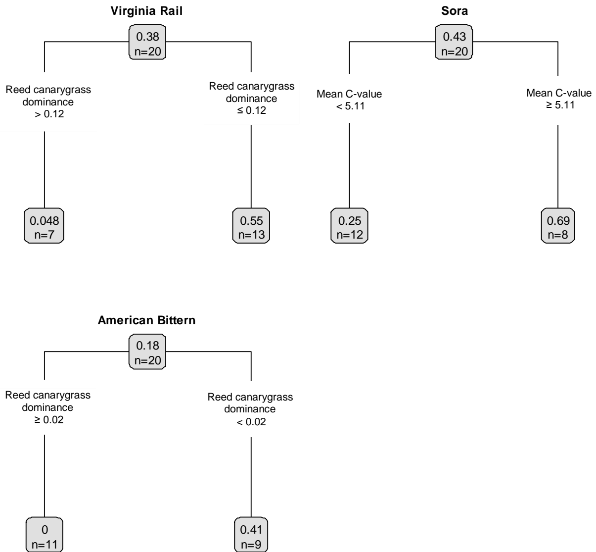
FIG. 3. Pruned regression trees for Virginia Rail, Sora, and American Bittern. All variables across three levels of sampling intensity were included in tree construction ( N = 20 ; Appendix B). Boxes at tree nodes (leaves) show size of each group and mean proportion of years occupied. A minimum split value of N = 20 was used, constricting trees to a maximum of two branches. R^2 = 0.40 (Virginia Rail), 0.35 (Sora), and 0.39 (American Bittern).
